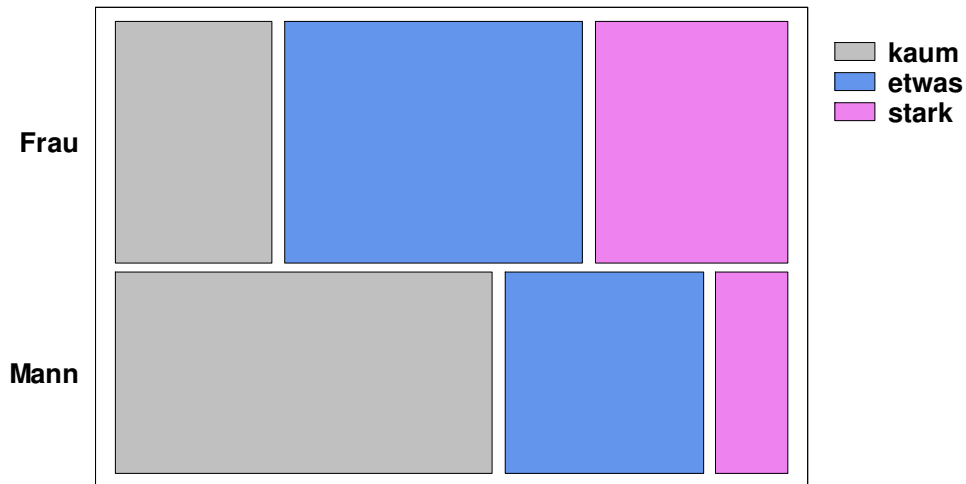
Mosaic Plot
