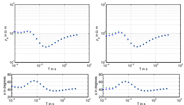
Fig. 4: Soundings of apparent resistivity \rho_a (top) and phase angle \phi (bottom) over a 100 \Omega\text{m} halfspace with an embedded 10 \Omega\text{m} layer between -200\text{ m} and -300\text{ m} depth, analytic '+' (green) and numeric 'o' (blue) solution, E- (left) and H- (right) Polarisation, max. error: \delta_{\rho_a} \leq 14\% , \delta_{\phi} \approx 2.8 degrees (left), \delta_{\rho_a} \leq 15\% , \delta_{\phi} \approx 5.4 degrees (right).
