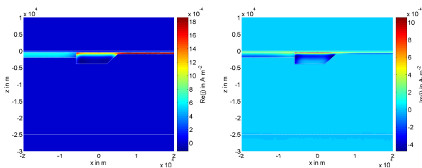
Fig. 7: Real (left) and imaginary (right) part of current density j_y , E-Polarisation.
