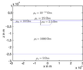
Fig. 5: COMMEMI model 2D-4.
