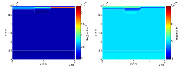
Fig. 8: Real (left) and imaginary (right) part of the current density j_x , H-Polarisation.
