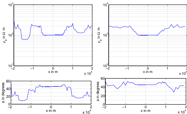
Fig. 3: Apparent resistivity \rho_a (top) and phase angle \phi (bottom) at the surface of a 100 \Omega\text{m} (left) and a 1000 \Omega\text{m} (right) halfspace at a frequency of f = 1\text{ kHz} , E-Polarisation, adaptive mesh refinement for -5000\text{ m} \leq x \leq 5000\text{ m} , error in adaptive refined region: \delta_{\rho_a} \leq 2.5\% , \delta_{\phi} \approx 0.7 degrees (left), \delta_{\rho_a} \leq 1.5\% , \delta_{\phi} \approx 0.5 degrees (right).
