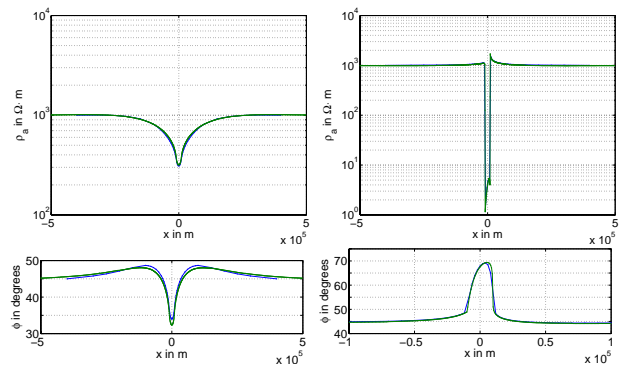
Fig. 10: Apparent resistivity \rho_a (top) and phase angle (bottom) \phi for the dike model (Fig. 9) computed by the FE (green) and the FD (blue) code at a frequency of f = 0.01 Hz, E- (left) and H-Polarisation (right), deviations: \Delta\rho_a \leq 6\% , \Delta\phi < 1.6 degrees, within the dike: \Delta\rho_a \leq 20\% , \Delta\phi \leq 3.2 degrees.
