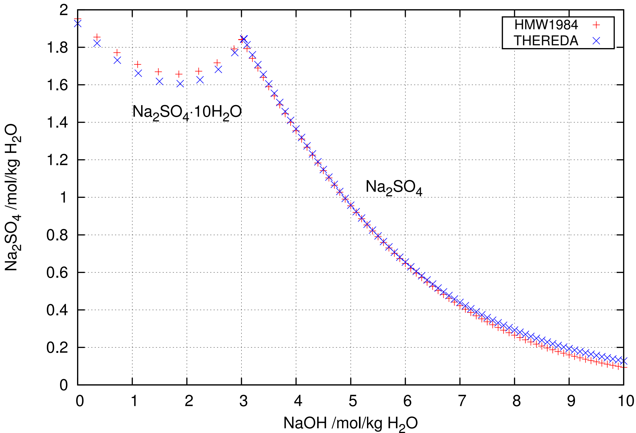
Solubility of \text{Na}_2\text{SO}_4 in solutions of \text{NaOH} at T=298.15 K
