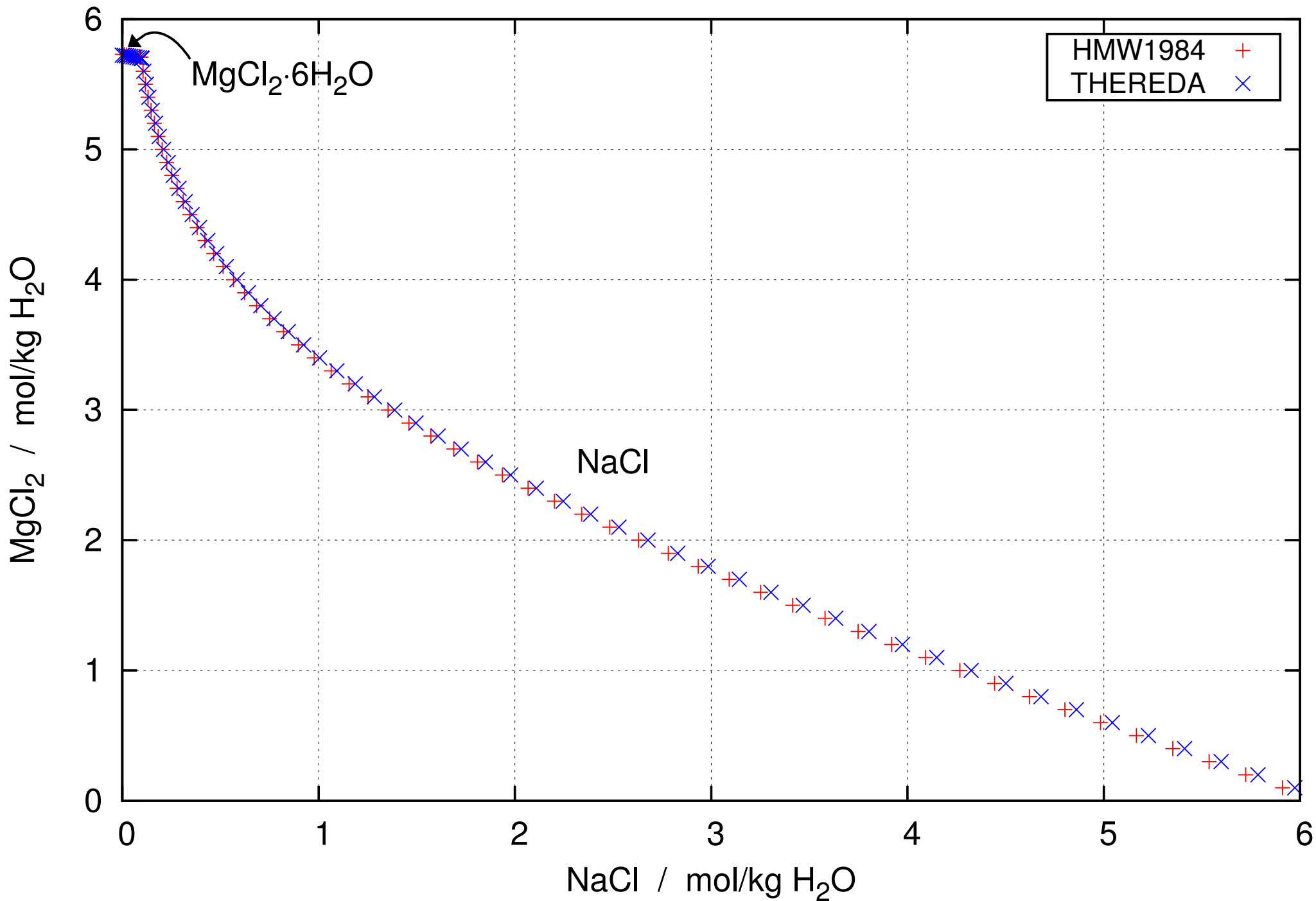
System NaCl-MgCl 2 -H 2 O at 298.15 K
