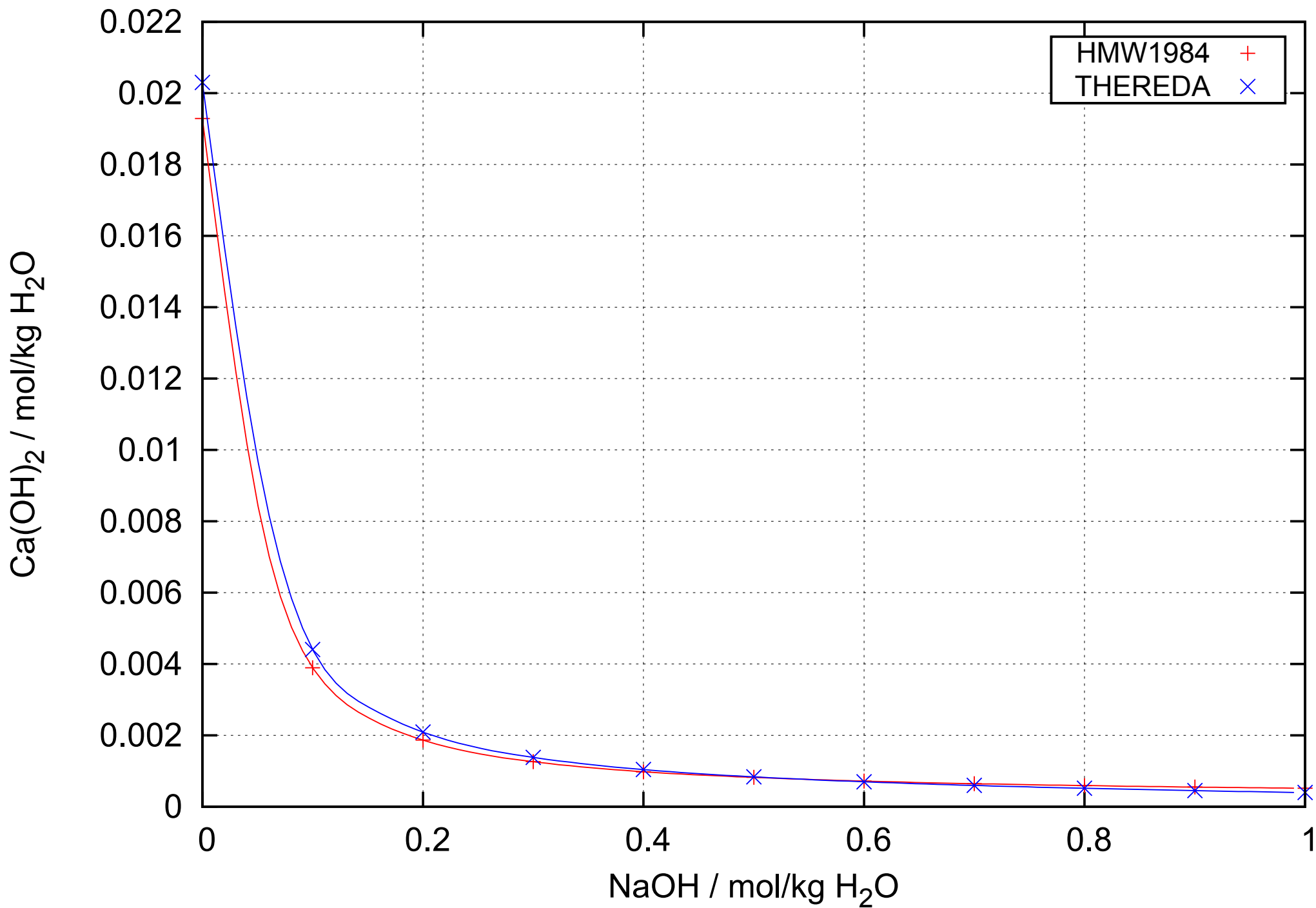
Solubility of \text{Ca}(\text{OH})_2 in dependence on \text{NaOH} concentration at T = 298.15 \text{ K}
