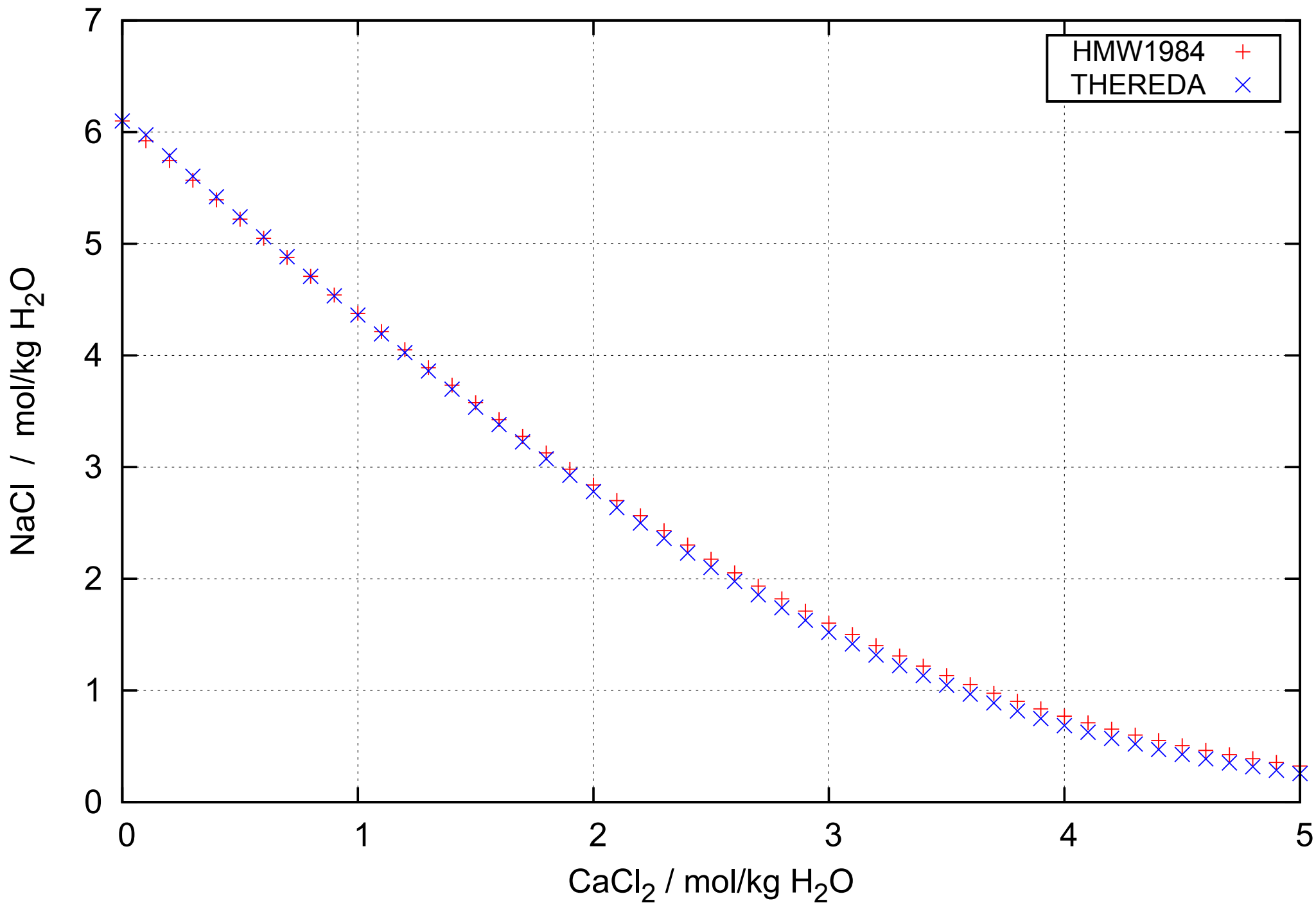
Solubility of NaCl in dependence on \text{CaCl}_2 concentration at T = 298.15 \text{ K}
