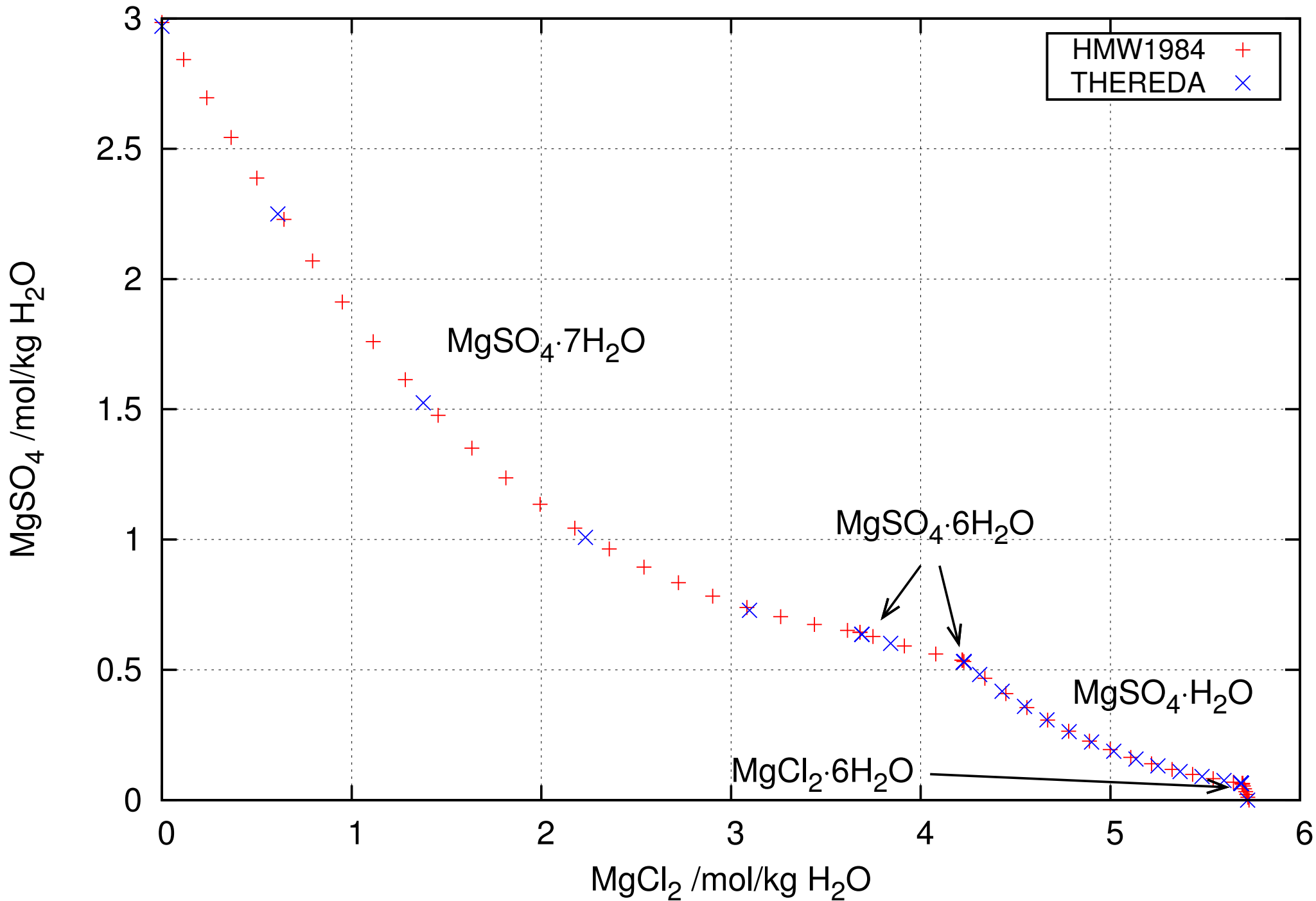
System \text{MgCl}_2\text{-MgSO}_4\text{-H}_2\text{O} at 298.15 K
