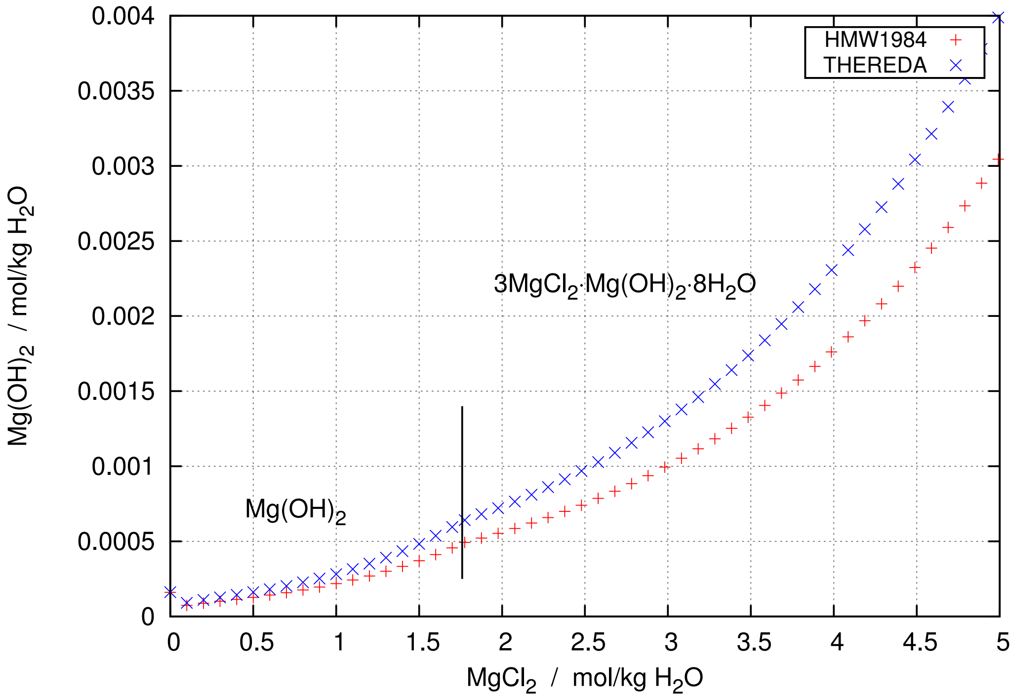
System \text{MgCl}_2\text{-Mg(OH)}_2\text{-H}_2\text{O} at 298.15 K, solubility of brucite
