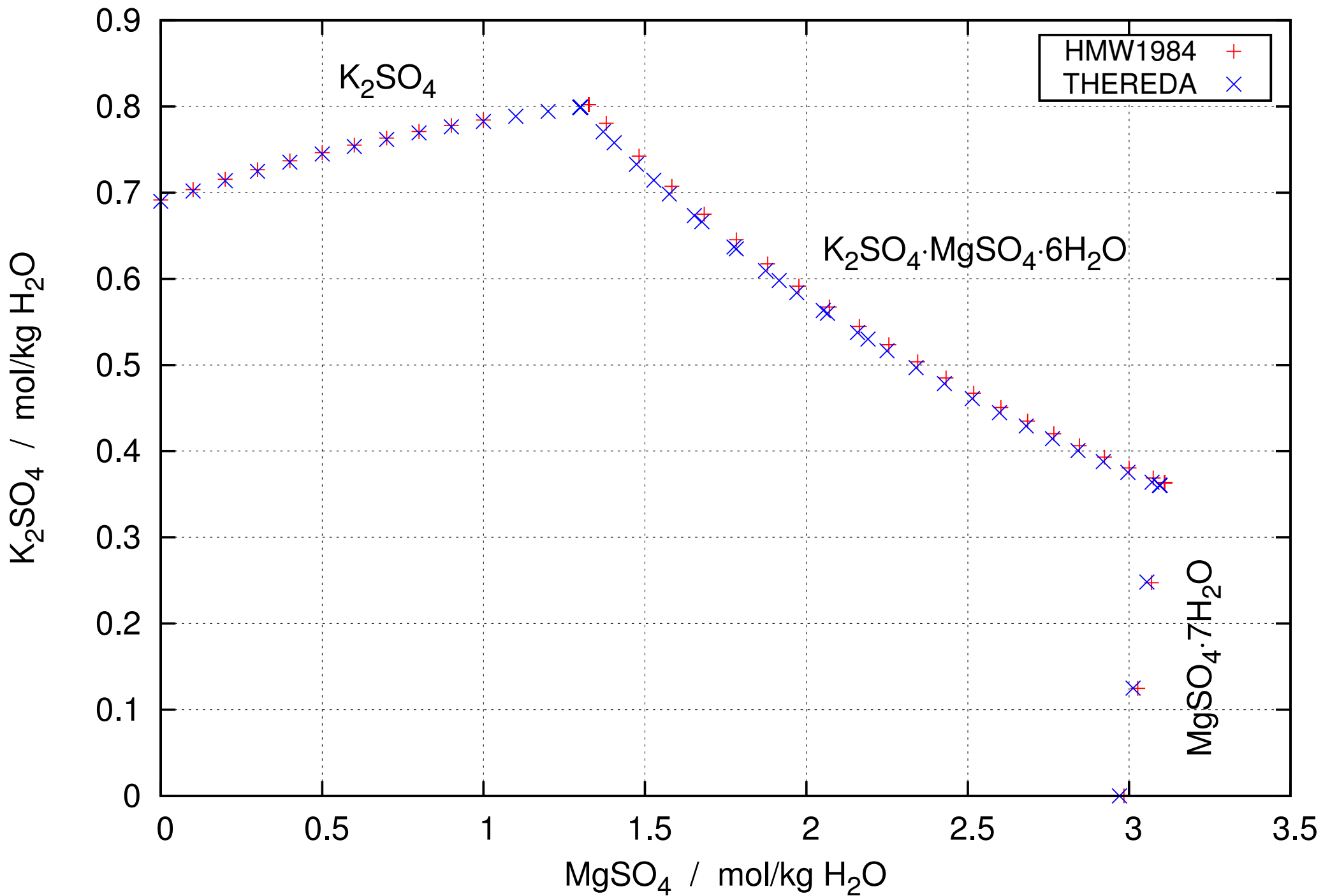
System \text{K}_2\text{SO}_4\text{-MgSO}_4\text{-H}_2\text{O} at 298.15 K
