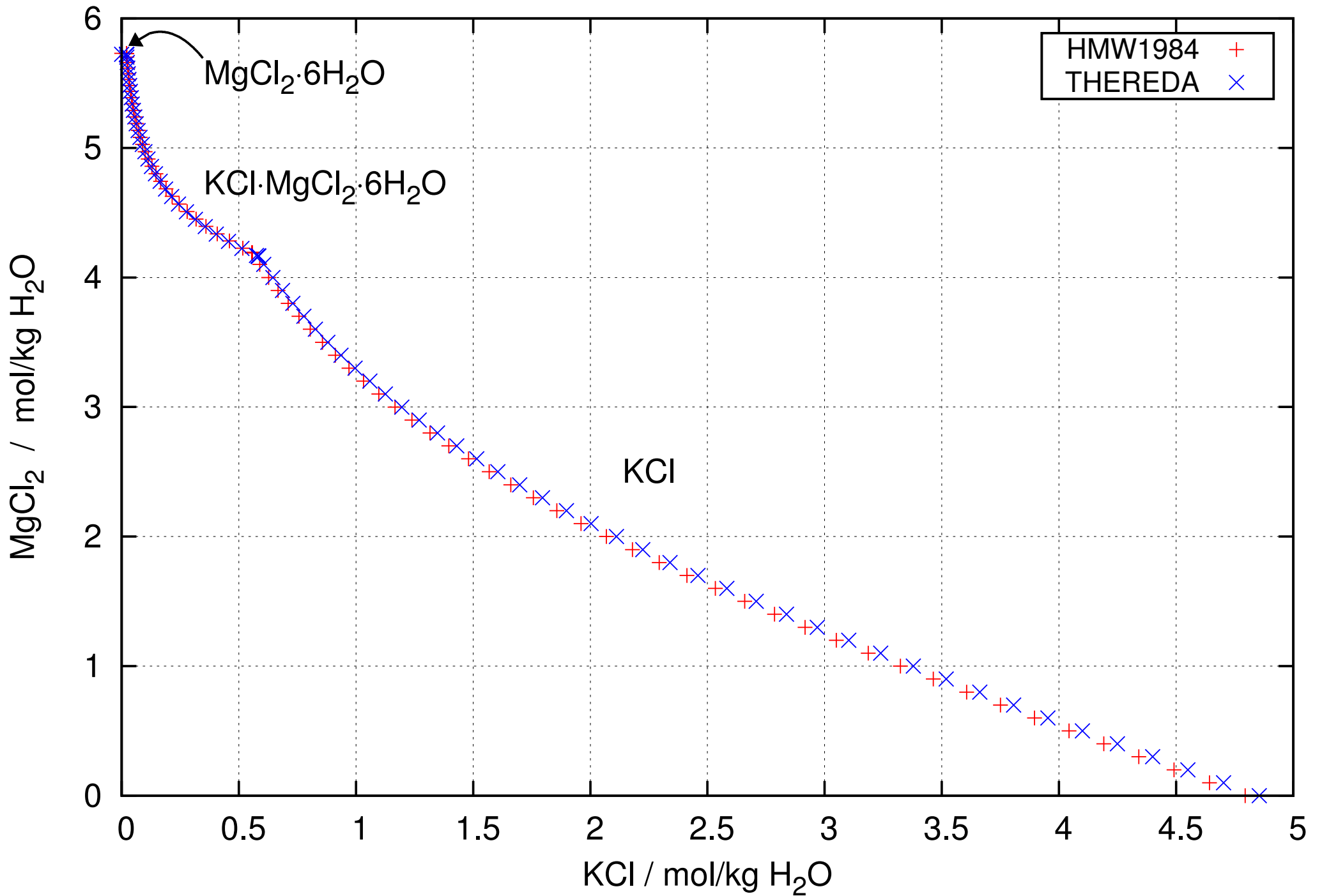
System KCl-MgCl 2 -H 2 O at 298.15 K
