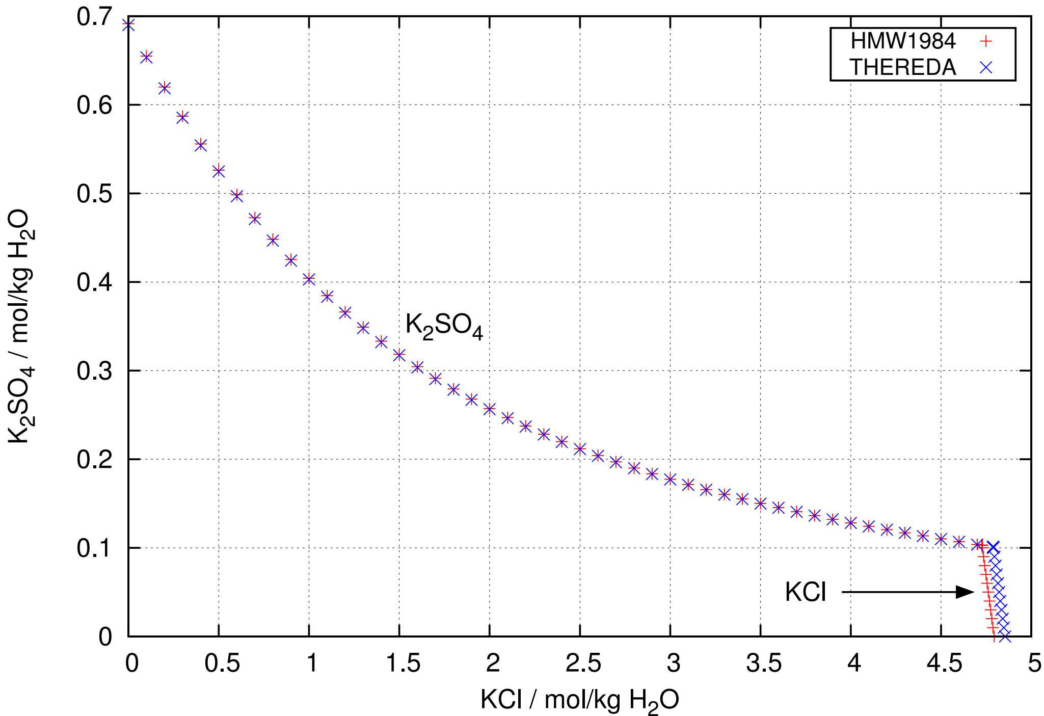
System KCl-K 2 SO 4 -H 2 O at 298.15 K
