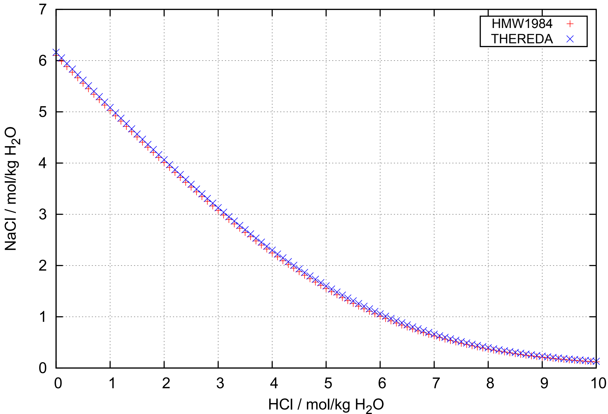
System HCl-NaCl-H 2 O at 298.15 K, solubility of NaCl
