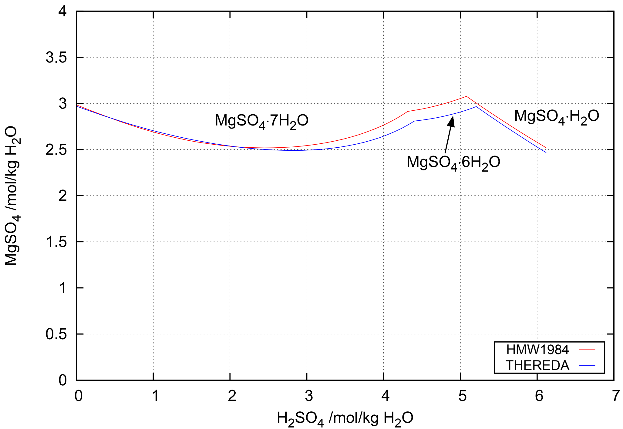
System \text{H}_2\text{SO}_4 - \text{MgSO}_4 - \text{H}_2\text{O} at T=298.15 K
