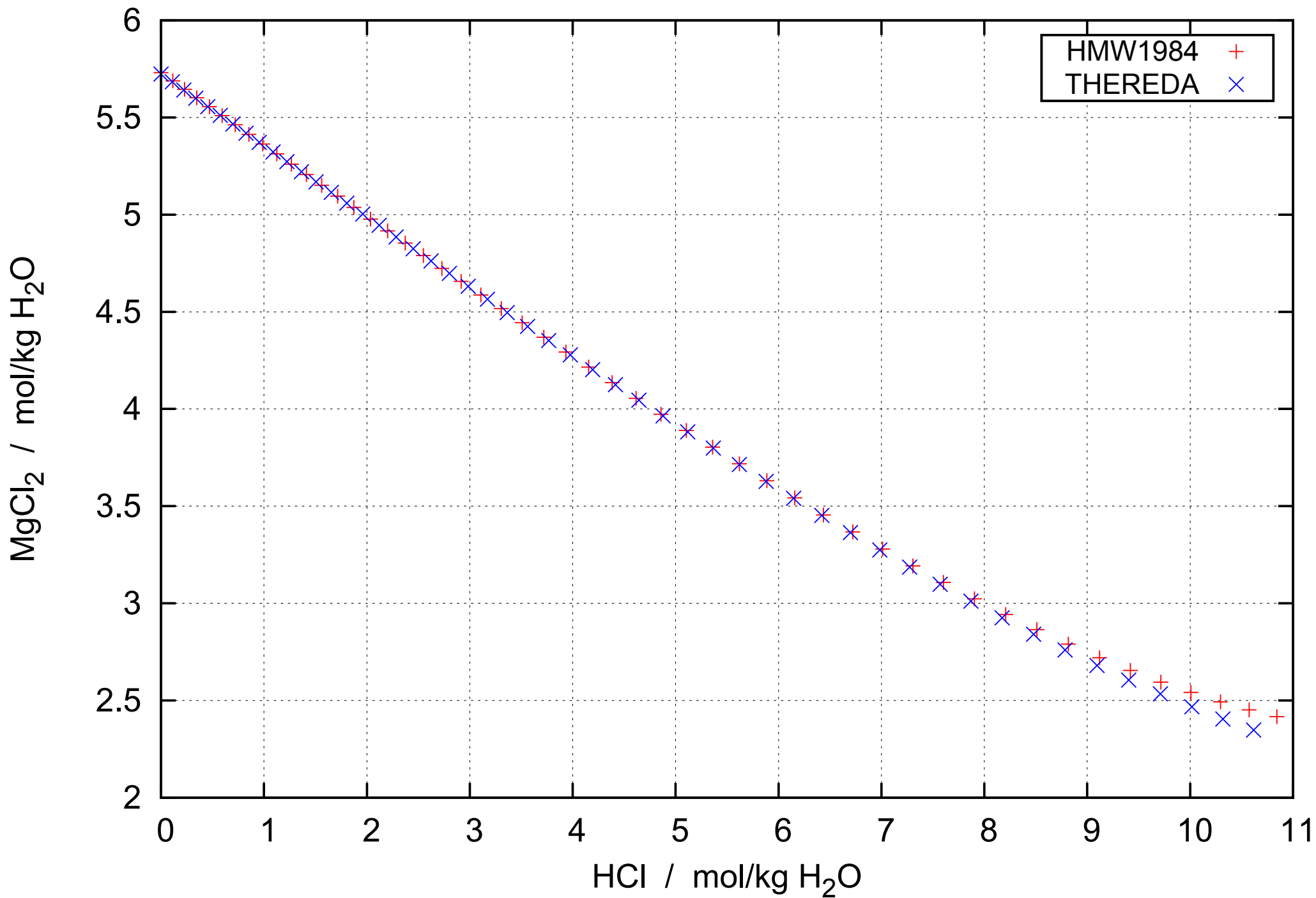
System HCl-MgCl 2 -H 2 O at 298.15 K, solubility of MgCl 2 ·6H 2 O
