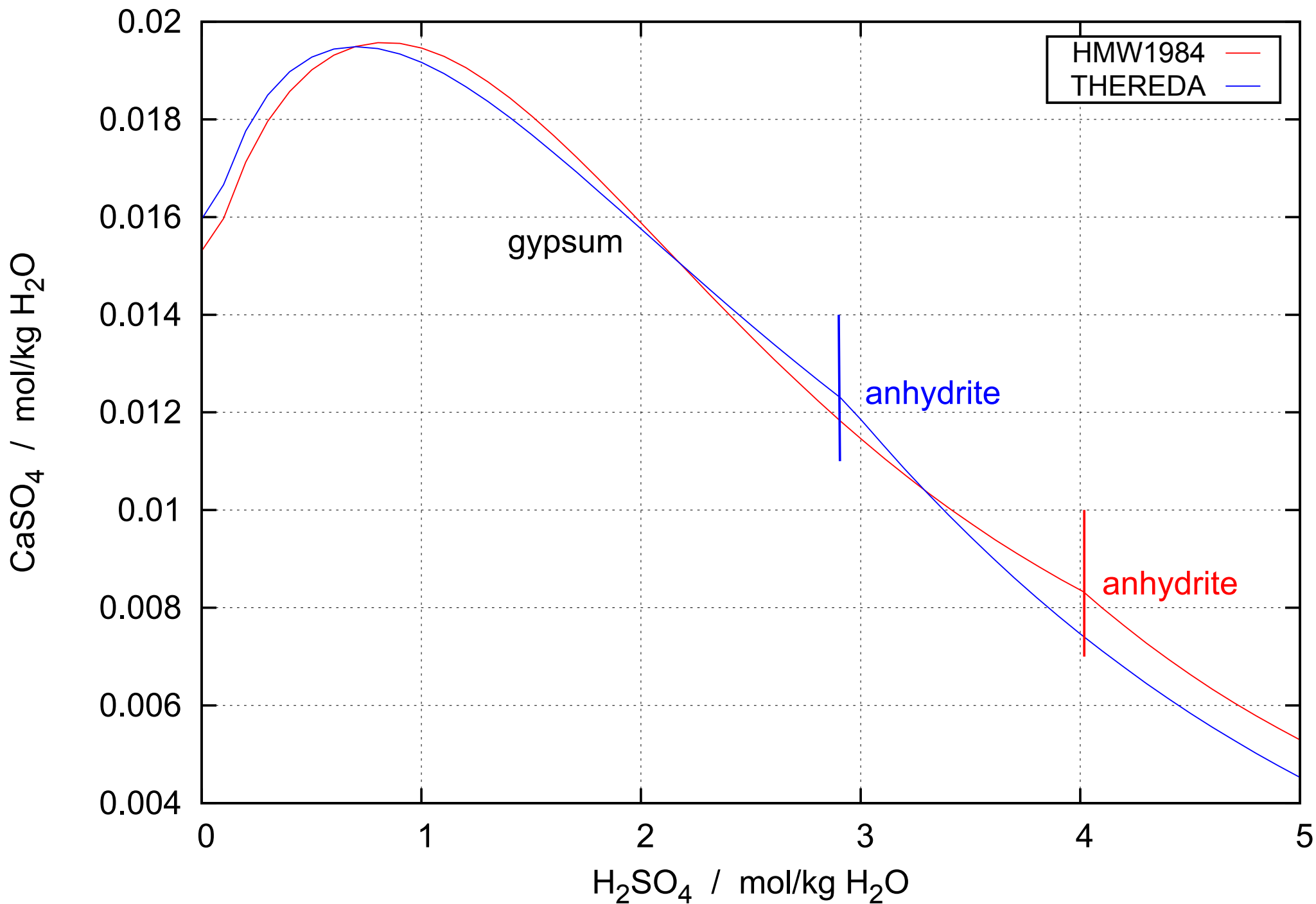
Solubility of \text{CaSO}_4 in sulfuric acid solutions at T = 298.15 \text{ K}
