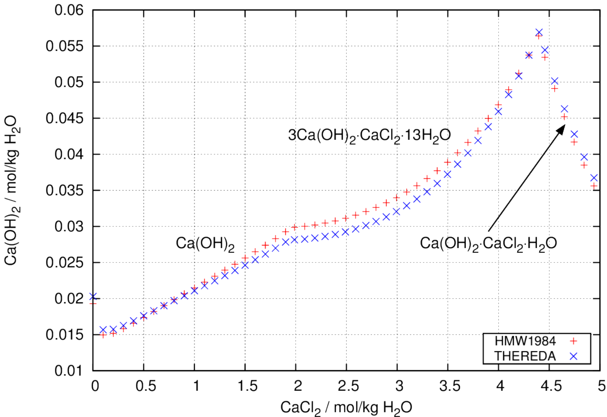
System \text{Ca}(\text{OH})_2\text{-CaCl}_2\text{-H}_2\text{O} at 298.15 K
