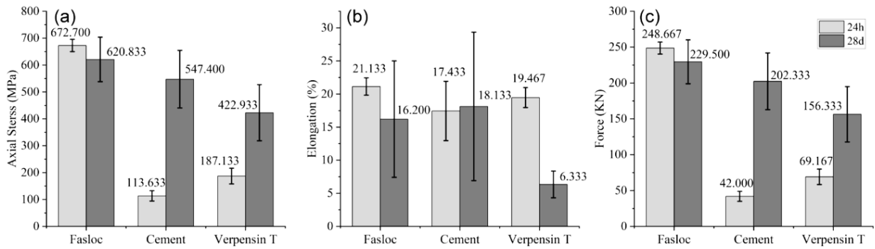
Fig. 5.4: Maximum pull-out force for fully grouted anchors after 24 hours and 28 days; bond types: Fasloc (resin), Verpensis (organic mineral glue) and Cem (portland cement), (Malkowski et al., 2023)
