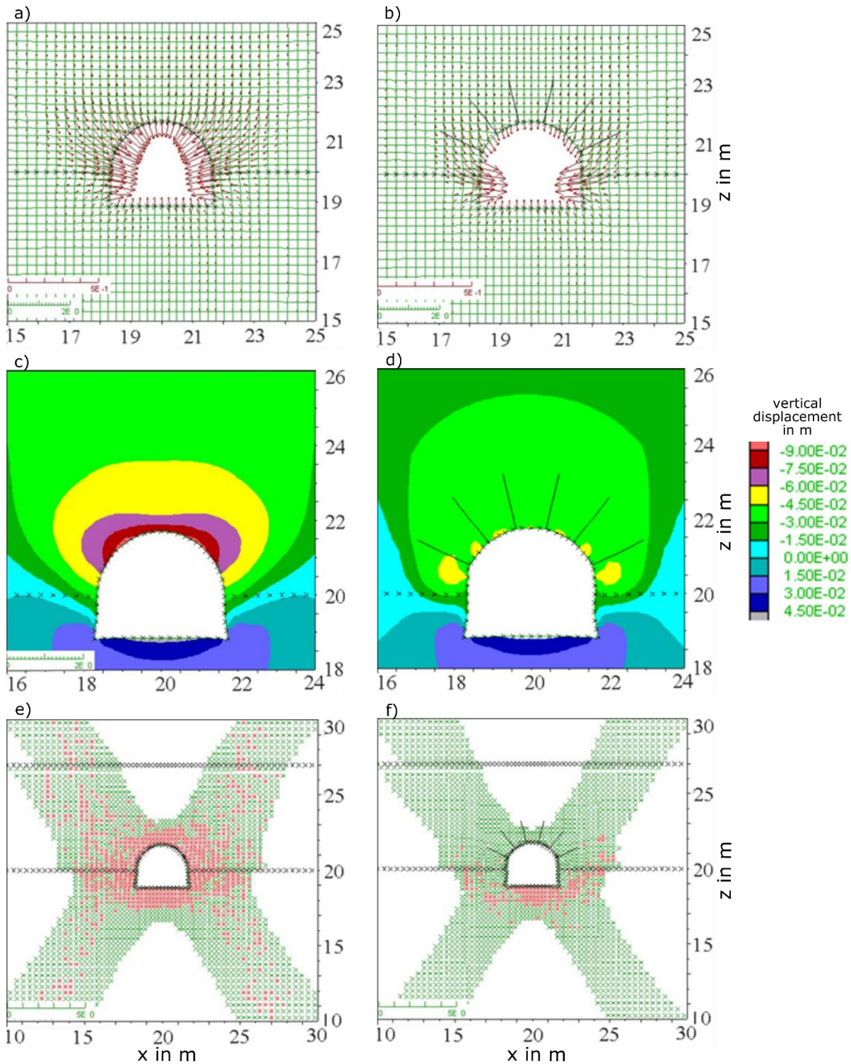
Fig. 9.7: Comparison between bolted and unbolted drift: a)+b): displacement vectors, c)+d): contours of vertical displacement magnitude, e)+f): plasticity state (red = active plastification) after Van (2008)
