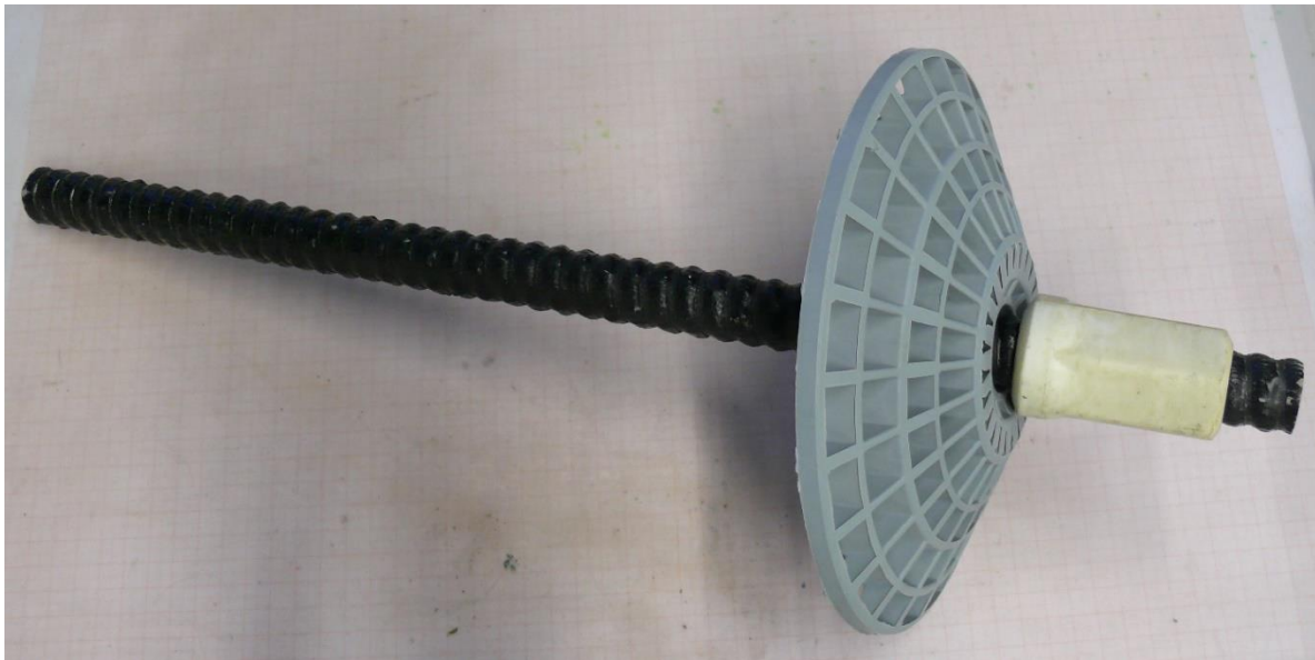
Fig. 4.8: GRP-anchor
