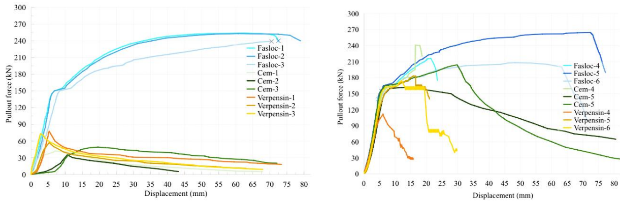
Fig. 5.3: Results from fully grouted pull-out tests after 24 hours (left) and 28 days (right); bond types: Fasloc (resin), Verpensis (organic mineral glue) and Cem (portland cement), (Malkowski et al., 2023)
