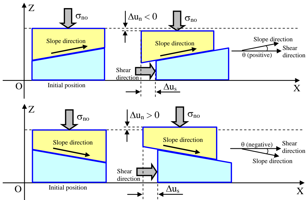
Fig. 3.14.6: Problem of 'apparent' dilation due to inclined fracture plane
