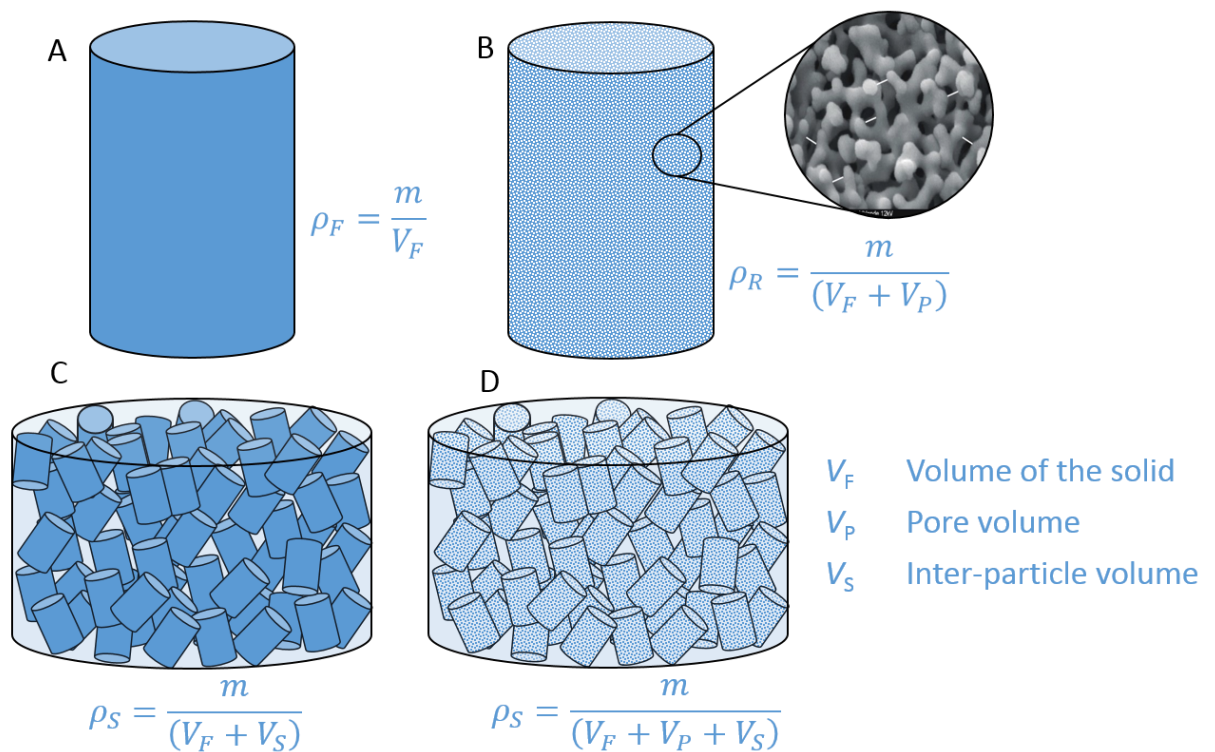
Fig. 8.2: Background of gas pycnometer measurements (company material)
