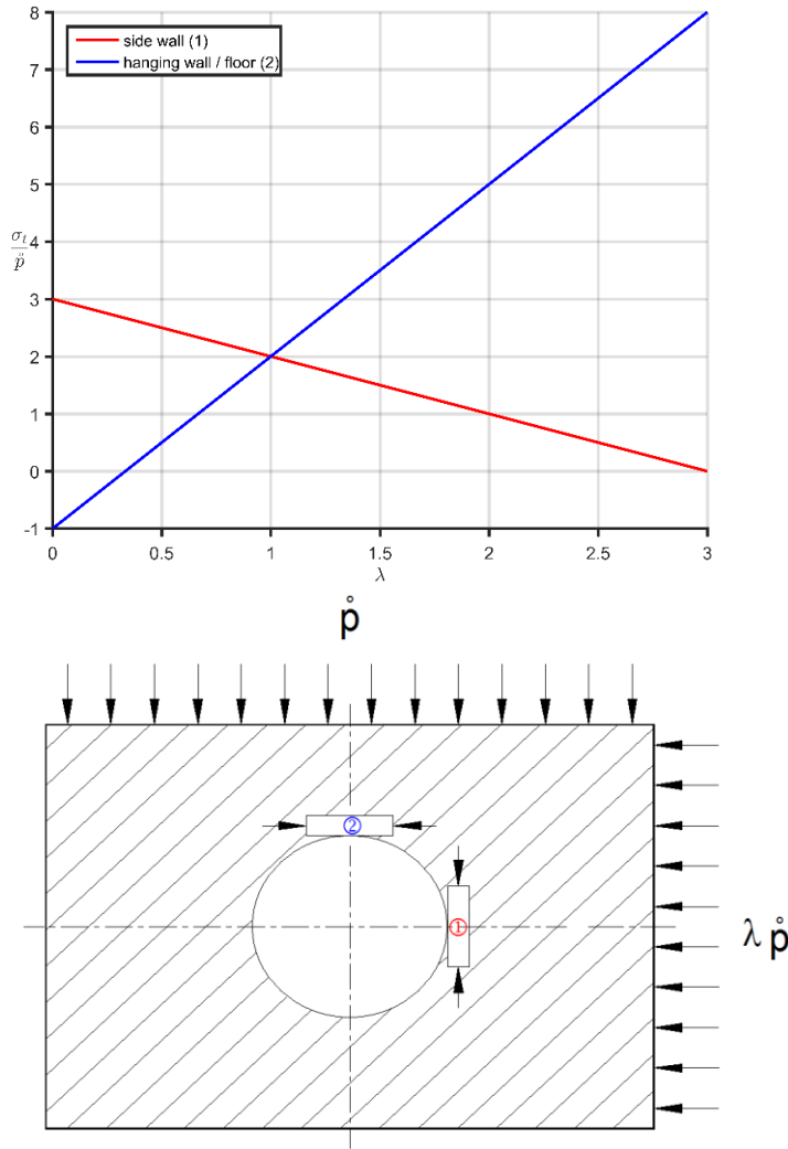
Fig. 7: Scaled tangential stresses vs. earth pressure coefficient at locations of extreme values
