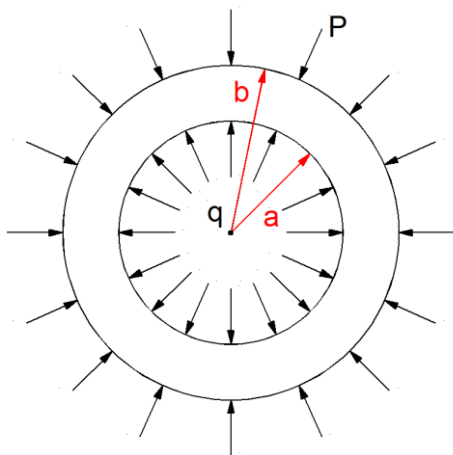
Fig. 12: Illustration of Lamé formulae
