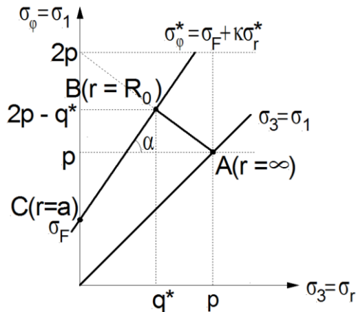
Fig. 17: Stress values (from A: far-field over B: boundary elastic-plastic region to C: boundary of opening) in principal stress diagram
