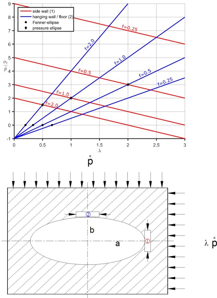
Fig. 14: Scaled tangential stresses at contour of elliptical opening with different elliptical axis ratio vs. earth pressure coefficient
