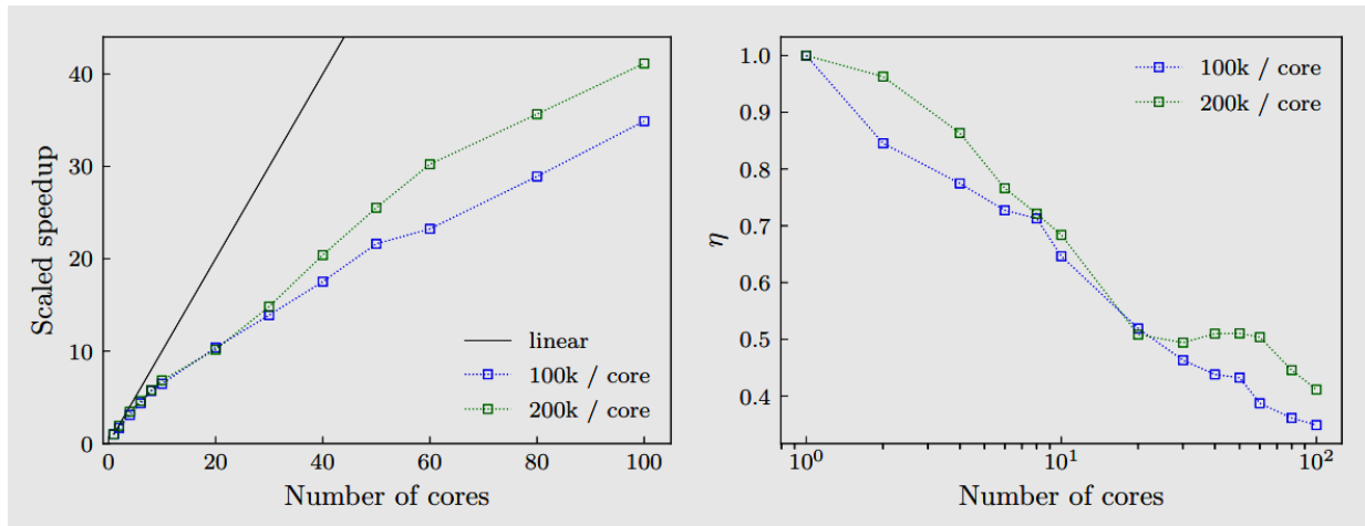
Fig. 11.4: Performance scaling on a HPC cluster for growing problem size, left: speed-up vs. number of cores for mesh with 100.000 or 200.000 zones per core, right: corresponding efficiency (Finenko, 2022)
