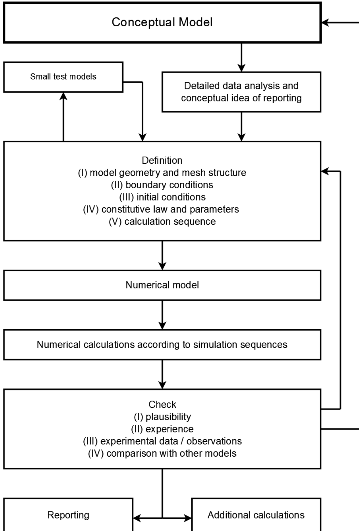
Fig. 14.2: Numerical model workflow
