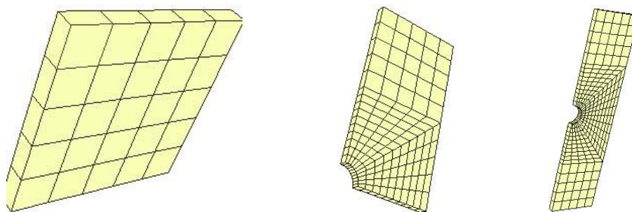
Fig. 4.2: Assemblage of subnets via docking and mirroring
