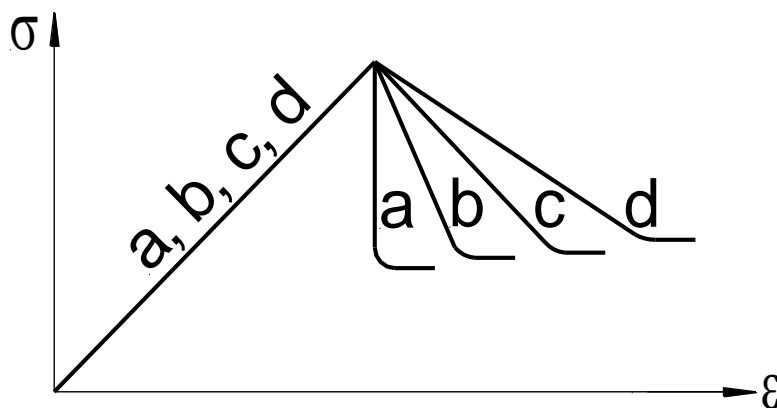
Fig. 10.1: Stress-strain behavior with strain-softening and different mesh refinement a,b,c and d without any procedure to avoid influence of mesh dependency
