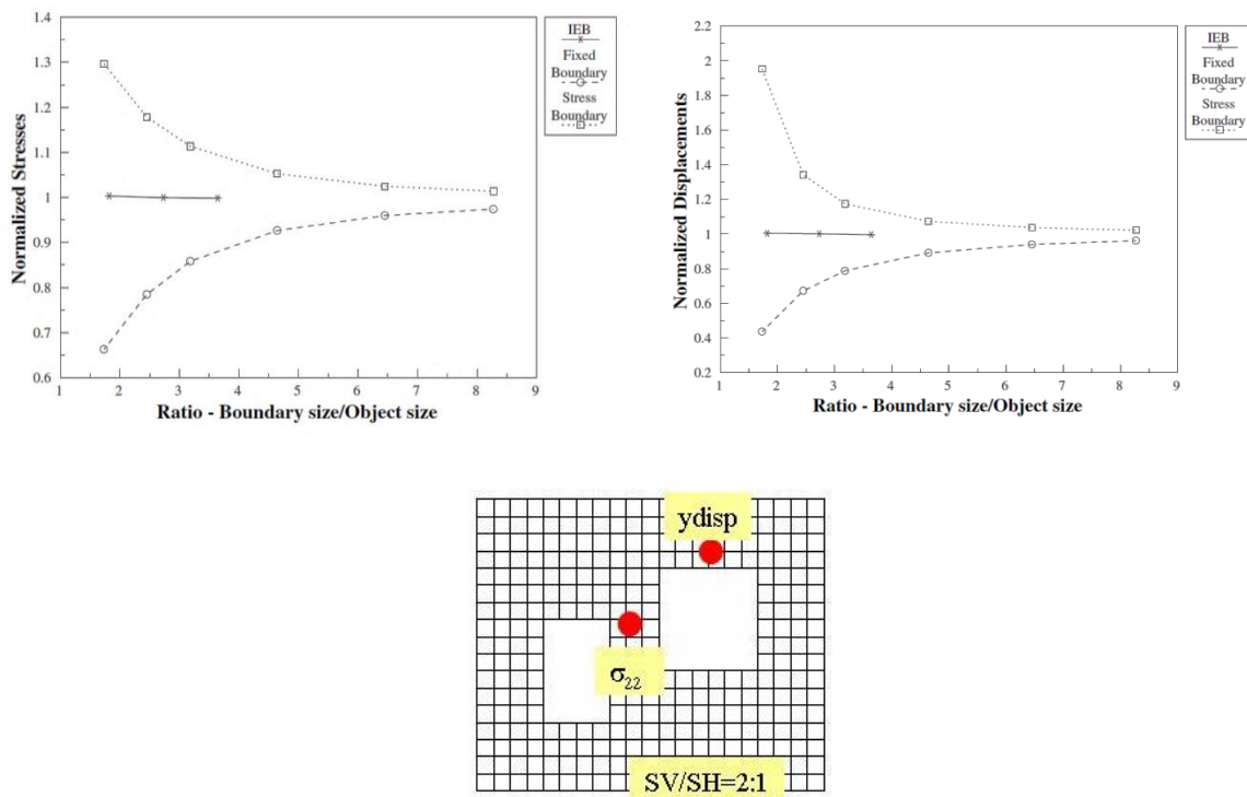
Fig. 2.1: Normalized stresses and displacements at two observation points in dependence of the type of boundary condition and the ratio of model size to excavation size [ITASCA 2011]
