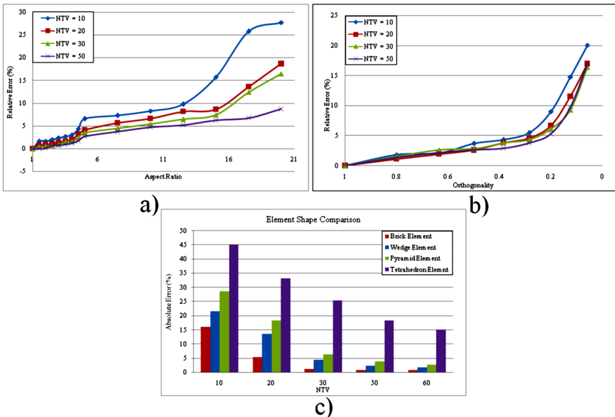
Fig. 5.1: Calculation error (radial stress) in respect to mesh parameters: (a) relative error vs. aspect ratio, (b) relative error vs. orthogonality, (c) absolute error vs. NTV (= mesh density) for different element types (Abbasi et al. 2013)
