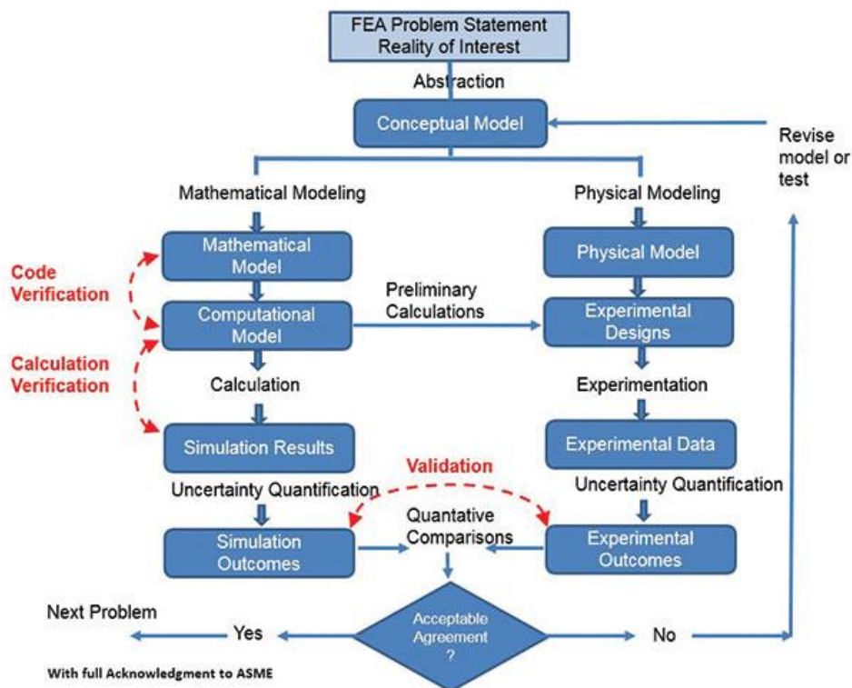
Fig. 15.2: Illustration of verification and validation (ASTM)
