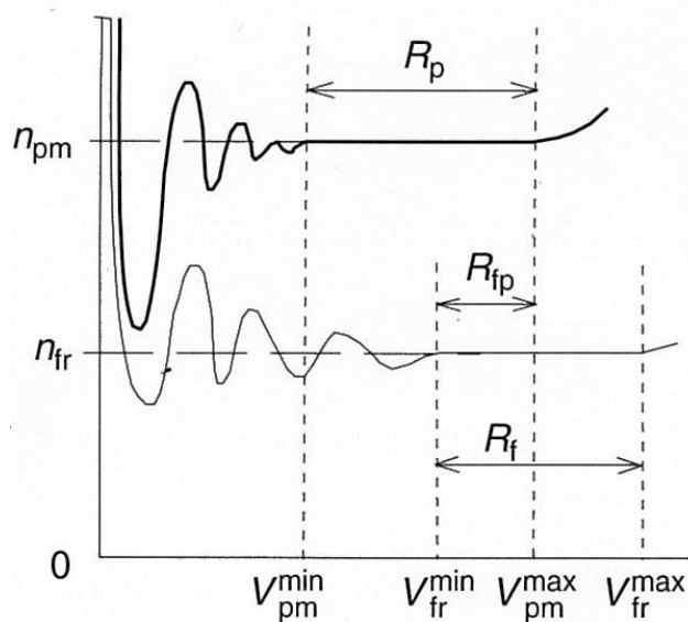
Fig. 7.1: Parameter history as function of considered volume (scale effect).
