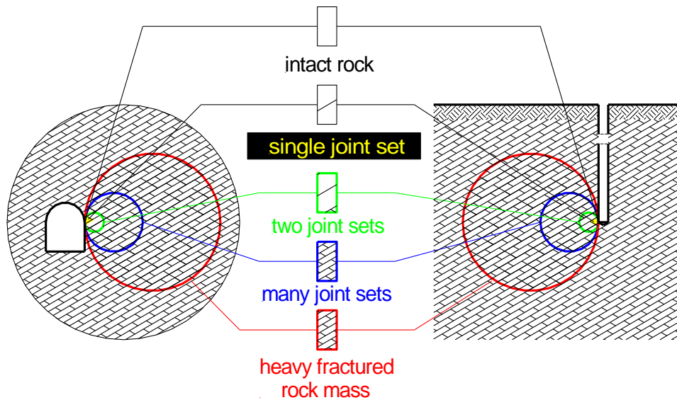
Fig. 7.2: Relation between structure and considered volume using the example of a rock mass (scale effect).
