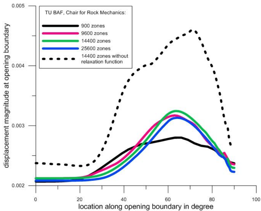
Fig. 10.3: Displacement magnitudes along tunnel contour vs. location of observation point
