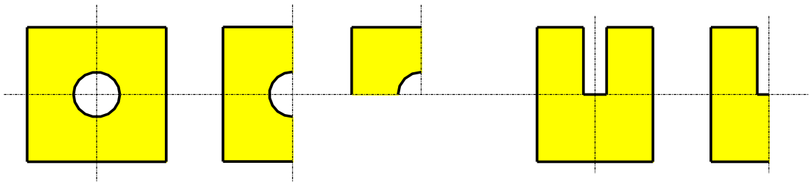
Fig. 8.1: Examples for model reduction on the basis of the consideration of pure geometrical symmetry conditions (full model, half model and quarter model)
