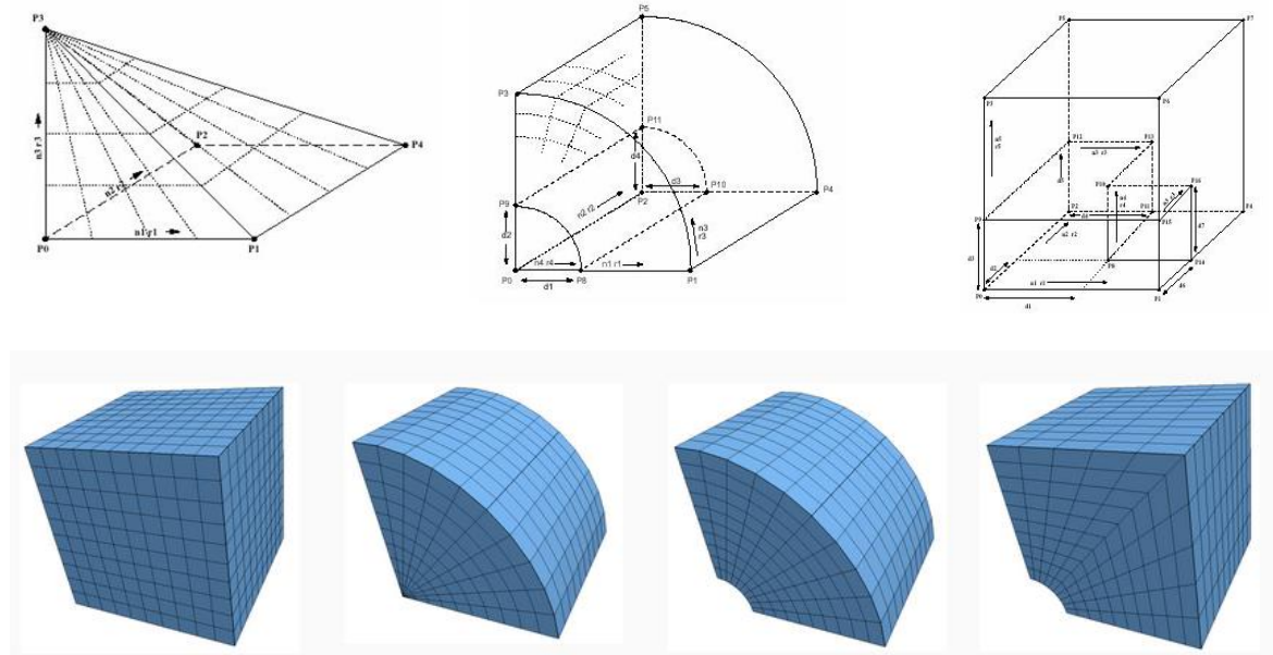
Fig. 4.1: Basic volumes filled with zones, which can be composed to a final model (‘LEGO-system’), (ITASCA 2012)
