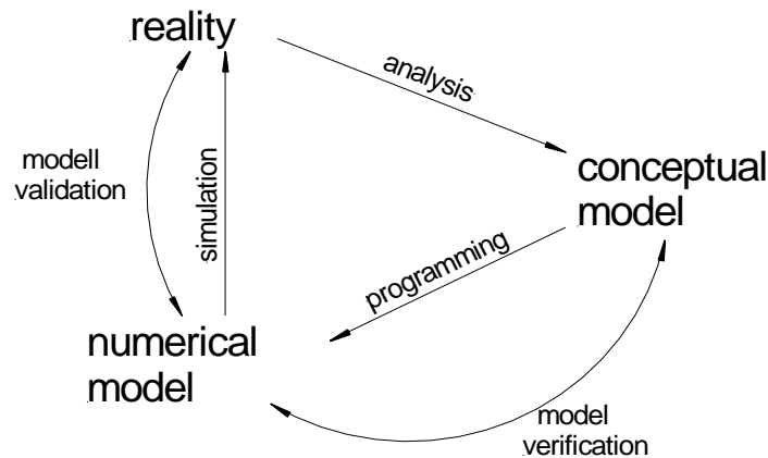
Fig.15.1: Role of verification and validation within the framework of simulation and software development
