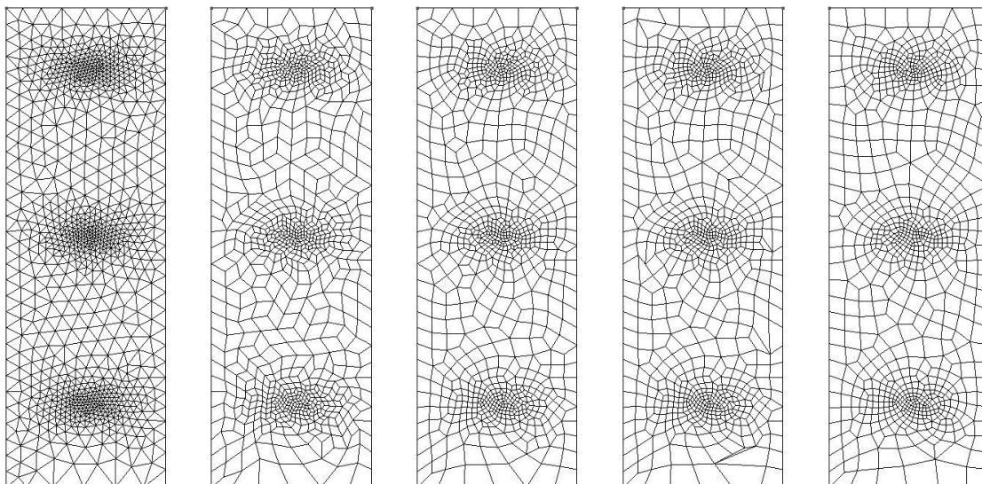
Fig. 4.8: Illustration of Blossom-Quad algorithm: transition from triangulation to quad-mesh (Remacle et al. 2010)
