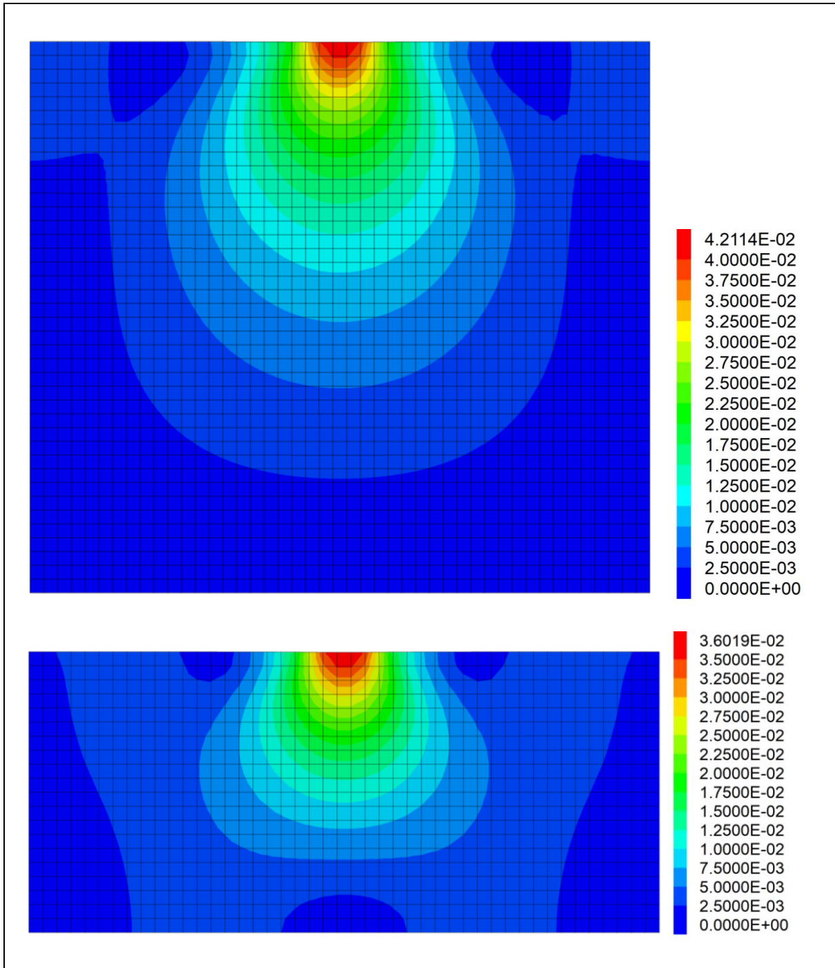
Fig. 6.2: Example: Influence of vertical model extension on the displacement magnitude (same conditions as documented in Fig. 6.1; horizontal extension is 45 m, vertical dimensions are: 40 and 20 m)
