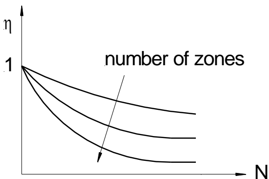
Fig. 11.2: Calculation efficiency \eta as function of number of processors N and number of zones
