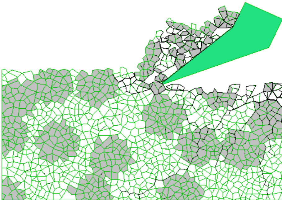
Fig. 13.1: DEM Simulation of cutting process for brittle rock (Lunow & Konietzky 2009)
