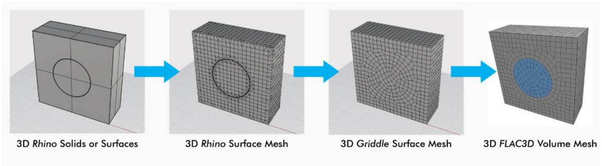
Fig. 4.4: Workflow from 3D CAD surface model to 3D volume mesh (Itasca, 2021)
