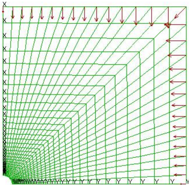
Fig. 10.2: Mesh for 1/4-symmetric tunnel including boundary conditions (900 zones)
