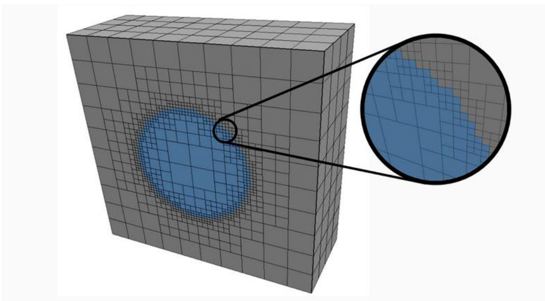
Fig. 4.6: Octree meshing (Itasca, 2021)
