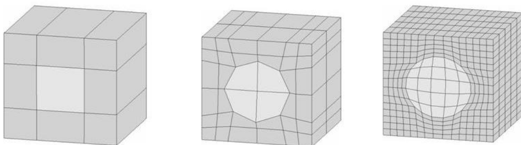
Fig. 4.3: Generation of final mesh by gradual geometrical adaption and mesh refinement
