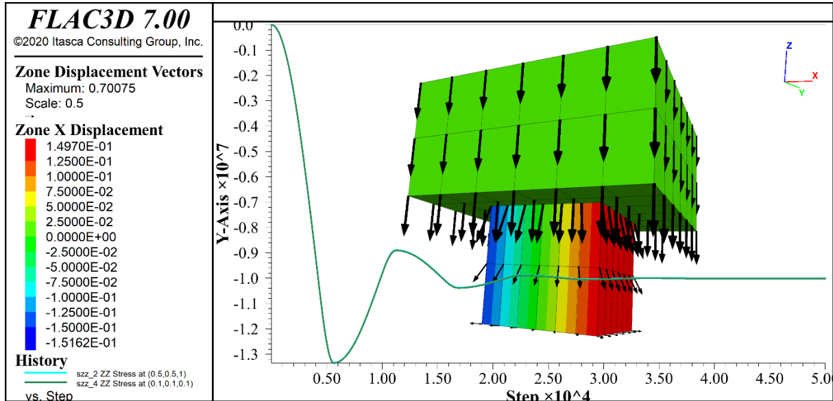
Fig. 12.1: Displacement vectors [m], horizontal displacement contours [m] and vertical stress evolution [Pa] in lower block using small strain modulus
