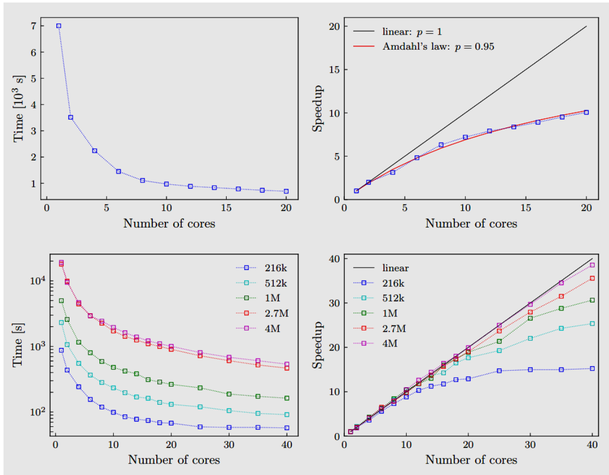
Fig. 11.3: Calculation performance on an HPC cluster for a fixed problem, top: calculation time and speed-up for a 2D mesh with 100.000 zones using different number of cores (note: p=f_p ), bottom: calculation time and speed-up for a 3D mesh with 216.000 to 4.000.000 zones using different number of cores (Finenko, 2022)
