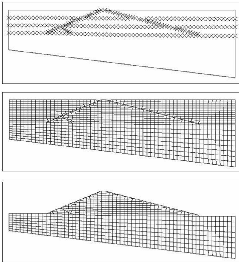
Fig. 4.7: Generation of final mesh via trimming, deformation and partial deletion of virigin (initial) mesh
