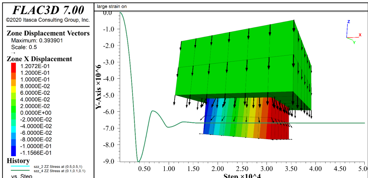
Fig. 12.2: Displacement vectors [m], horizontal displacement contours [m] and vertical stress evolution [Pa] in lower block using large strain modulus
