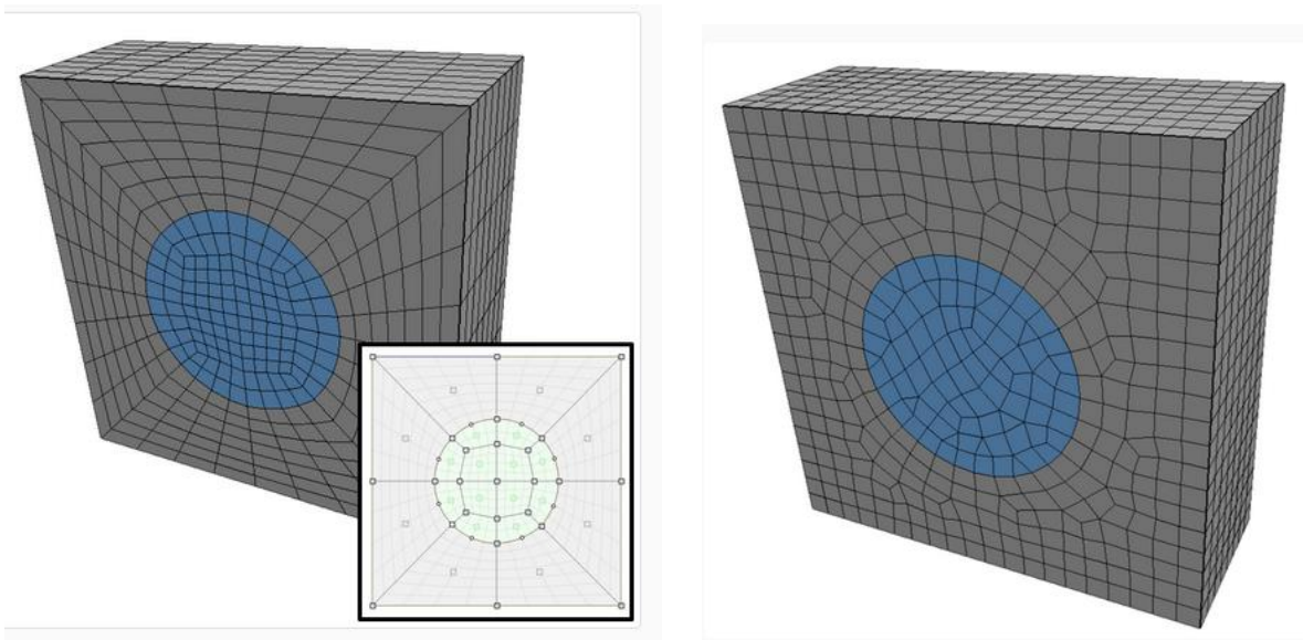
Fig. 4.4: Workflow from 3D CAD surface model to 3D volume mesh (Itasca, 2021)
