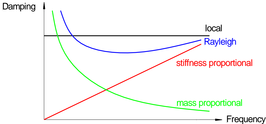
Fig. 8.1: Damping vs. frequency for different damping procedure
