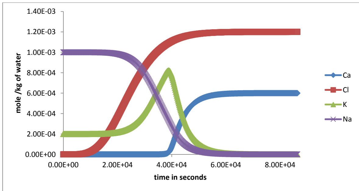
Figure 9.3a Simulation of cation exchange using VS2DRT
