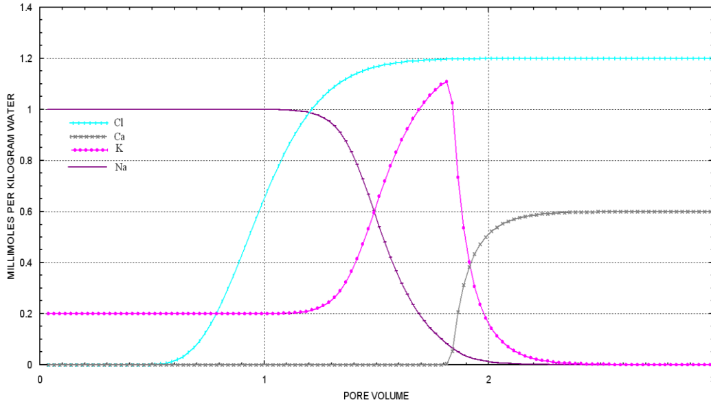
Figure 9.3b PHREEQC simulation of cation exchange involving advection and dispersion transport.
