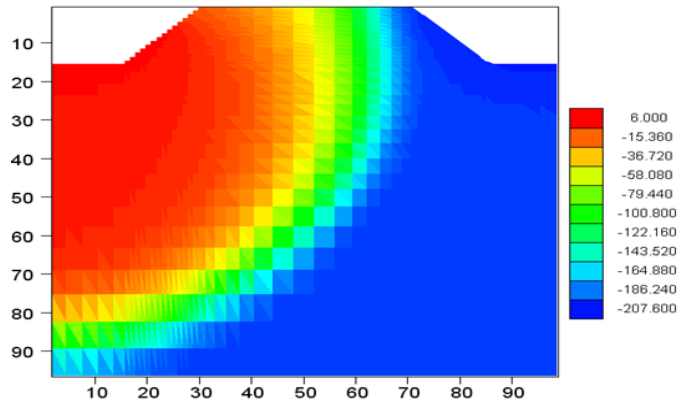
Figure 9.6b Pressure head profile at times a) 0.1, b) 0.5, c) 1 and d) 2 days using VS2DRT simulation
